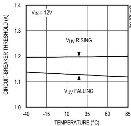
CIRCUIT-BREAKER THRESHOLD vs. TEMPERATURE
