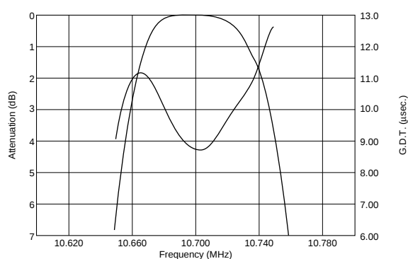
SFVLA10M7LF00-B0
