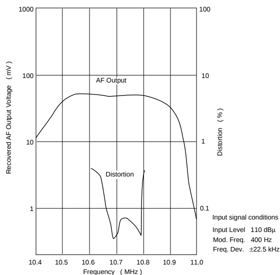
Frequency Characteristics
