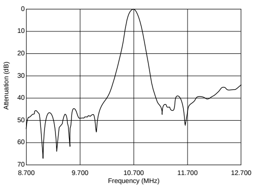
SFELA10M7HAXD-B0
