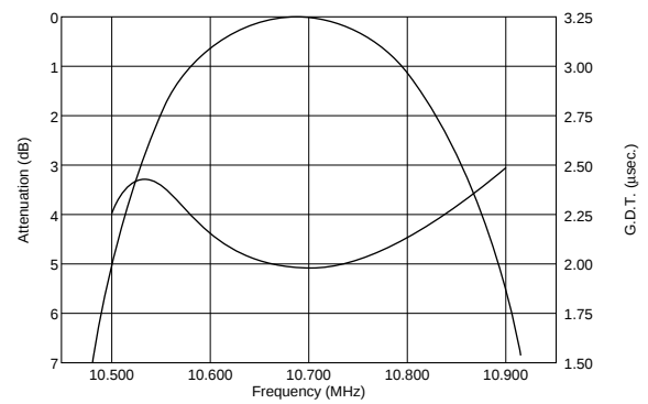
SFELA10M7FALL-B0
