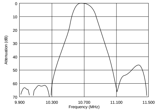
SFELA10M7HA0G-B0
