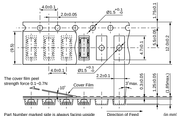
CDSCA Series
