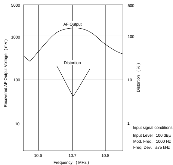
Frequency Characteristics
