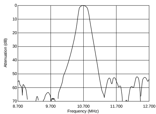
SFELB10M7FA00-B0
