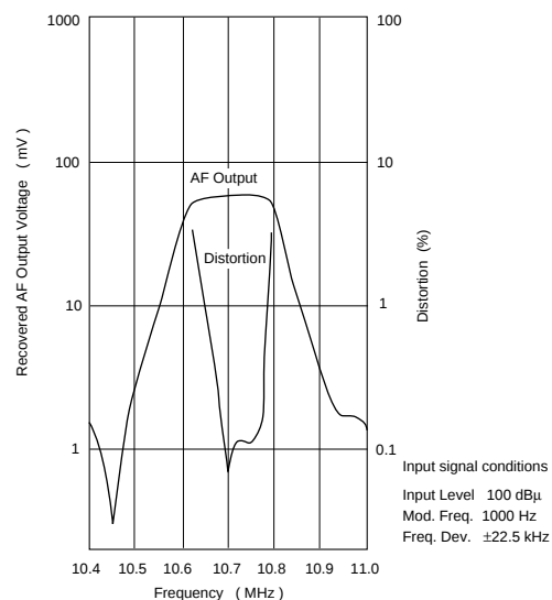
Frequency Characteristics
