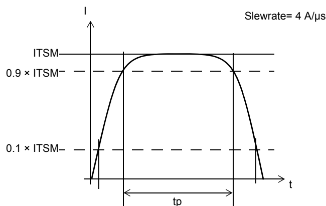
Figure 4-1 • 10 ms Surge Current Waveform
