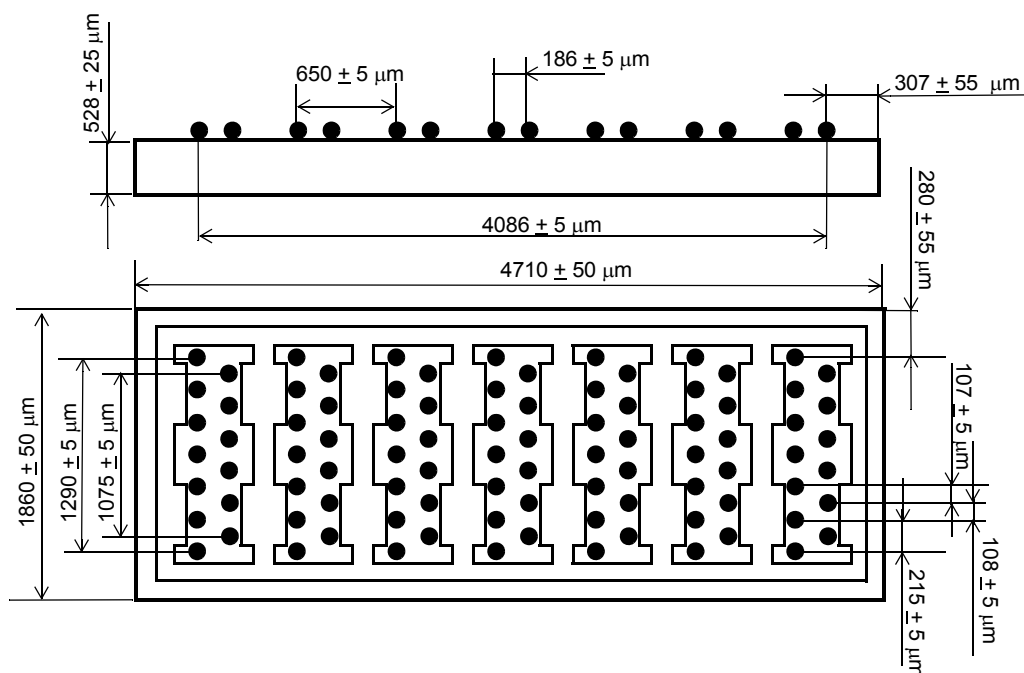
Figure 7-2 • Die Size and Bump Placement of ZL70574
