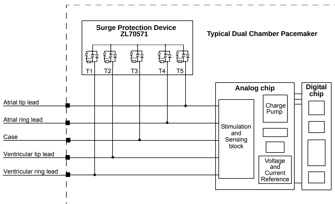
Figure 2-1 • Pacemaker Application Example
