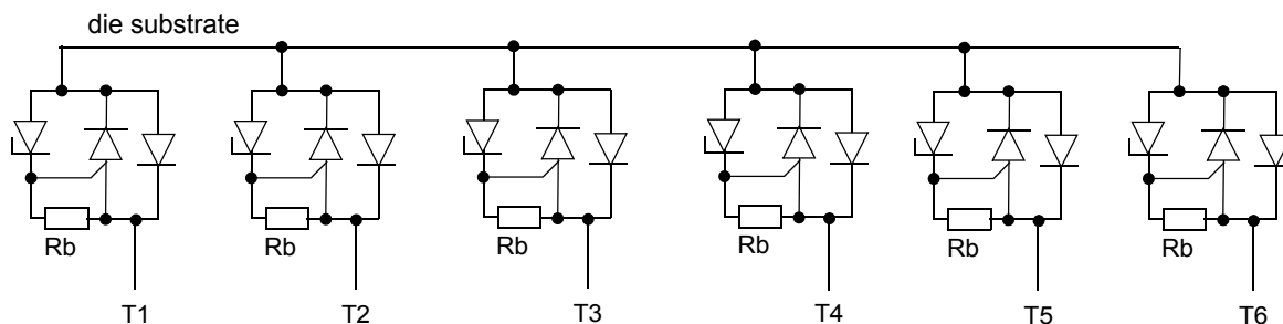
Figure 1 • ZL70573 Block Diagram
