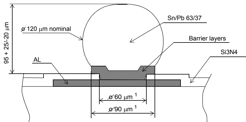
Figure 7-4 • Solder Bump Appearance of ZL70571/72/73/74
