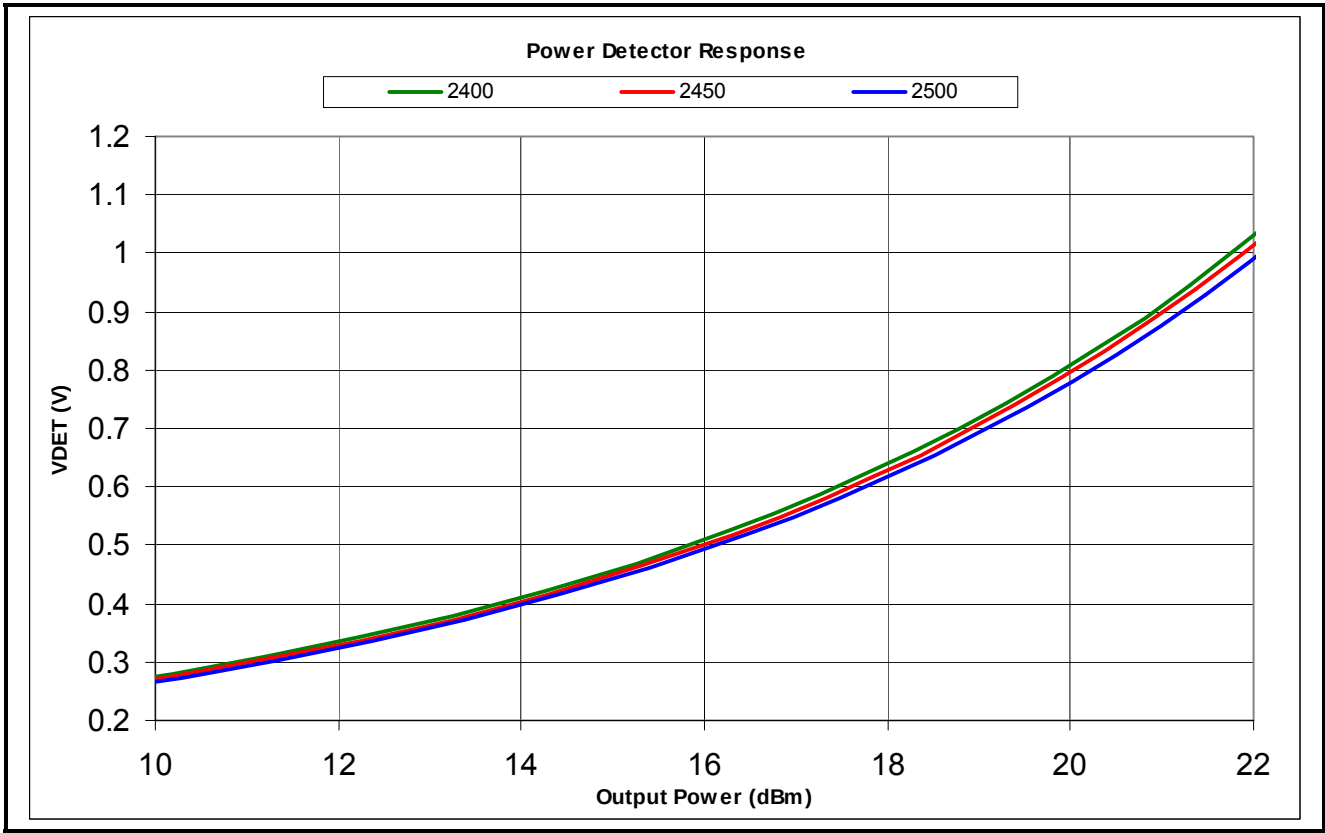
Figure 3: Power Detector Characteristic
