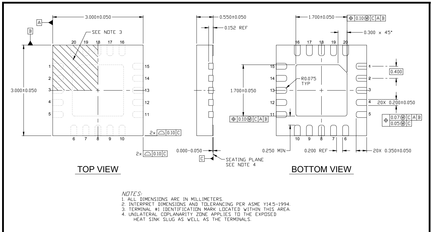
Figure 5: SE2611T Package Diagram
