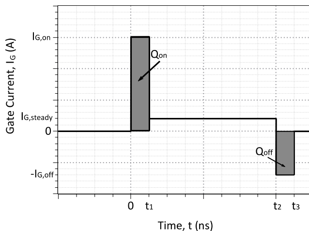
Figure 3: Idealized SGT Gate Current Waveform
