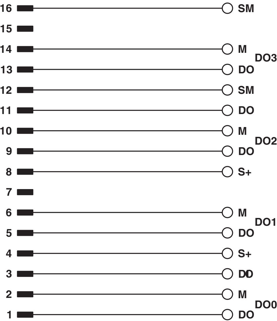
Circuit diagram
