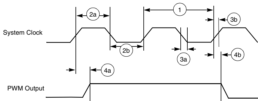
Figure 46. PWM Timing
