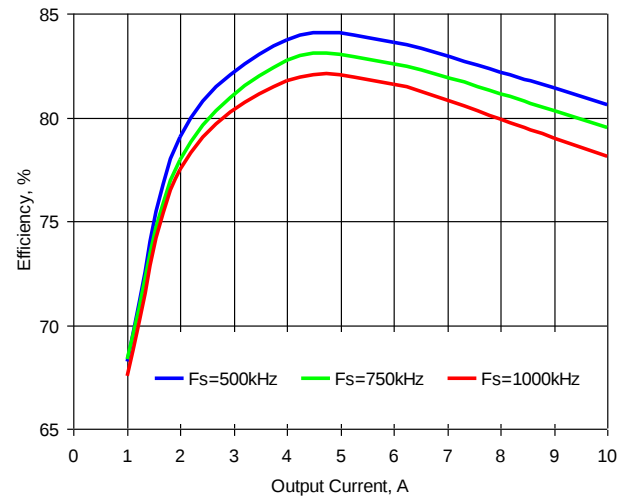
Figure 8. Efficiency vs. Load. Vin=5V, Vout=1.2V
