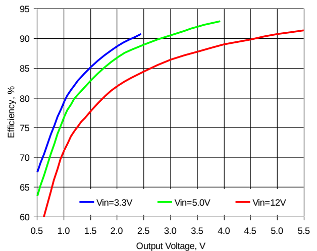
Figure 5. Efficiency vs. Output Voltage, Iout=10A, Fsw=500kHz
