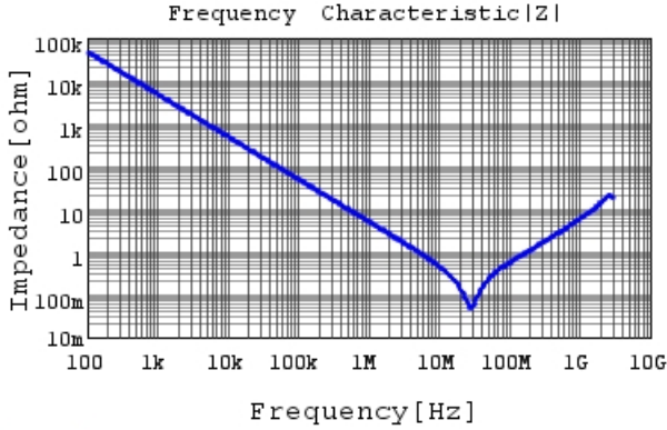
GRM31CR72E333KW03 |Z| DCOV, 25degC
