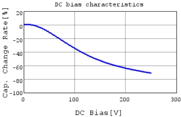
GRM31CR72E333KW03 C-DC bias capchange, 25.0c
