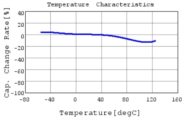
GRM31CR72E333KW03 C-Temp. capchange, DCOV, 1
