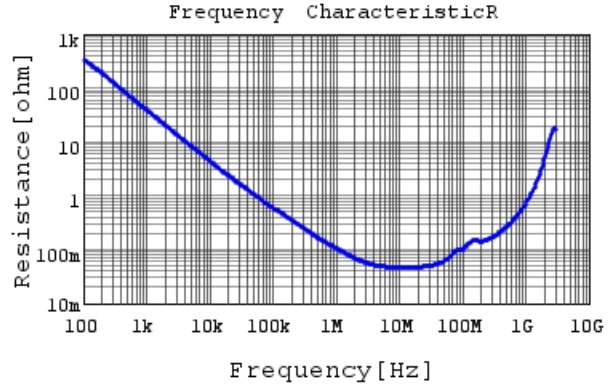
GRM31CR72E333KW03 R DCOV, 25degC
