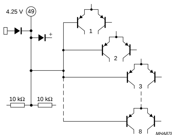
Fig.48 Pin 49: capacitor subwoofer.
