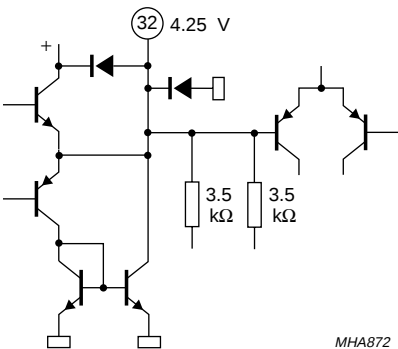
Fig.42 Pin 32: capacitor for pilot detector.
