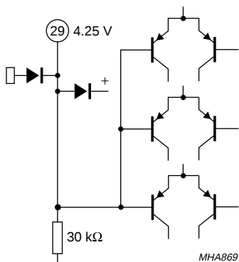
Fig.39 Pin 29: input composite signal.
