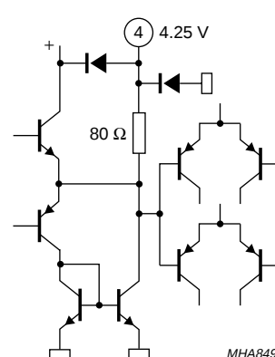
Fig.19 Pin 4: output subwoofer; pin 6: output, left channel; pin 14: output selector, left channel; pin 39: output selector, right channel; pin 47: output, right channel.
