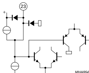
Fig.34 Pin 23: capacitor mute for SAP.
