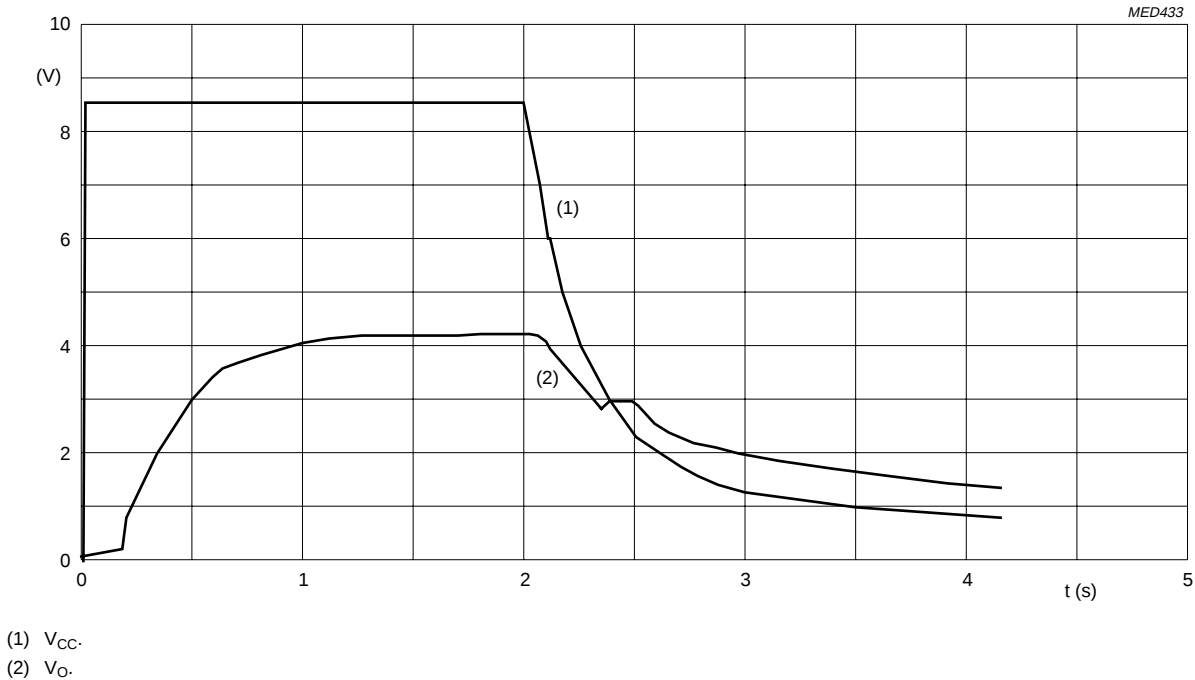
Fig.15 Turn-on/off behaviour.
