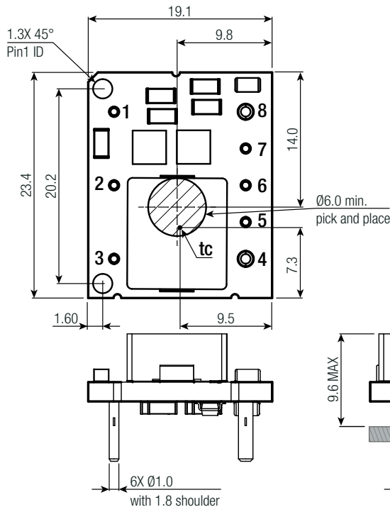
Dimension Drawing (mm)
