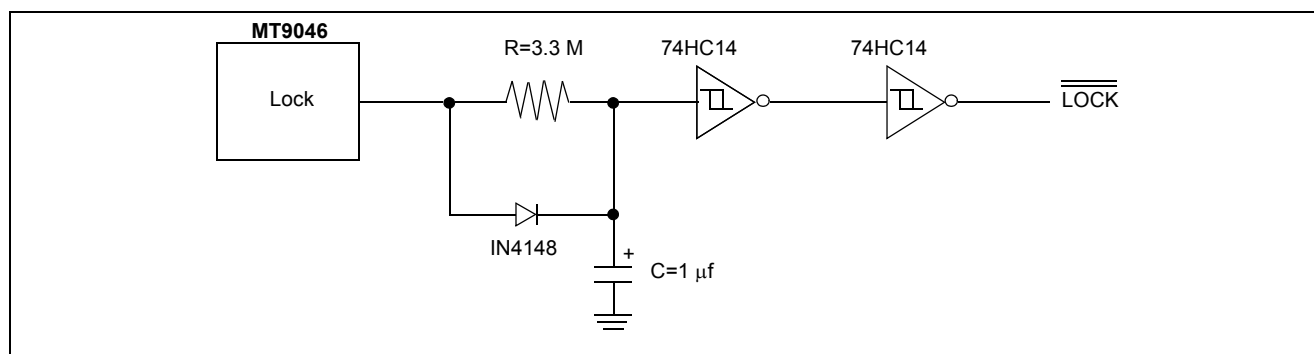
Figure 11 - Time-constant Circuit
