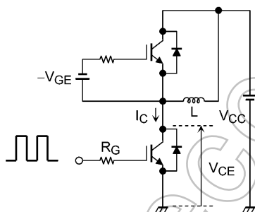
Fig. 6.2.1 Test Circuit of Switching Time
