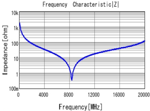
■ GCQ1555C1HR90WB01 |Z| DC0V, 25degC
