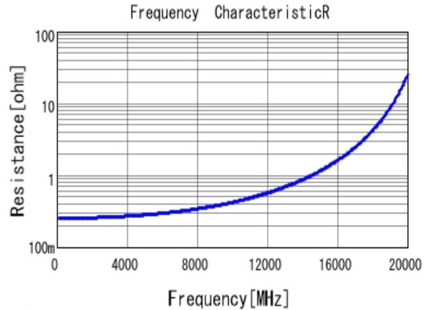
■ GCQ1555C1HR90WB01 R DC0V, 25degC
