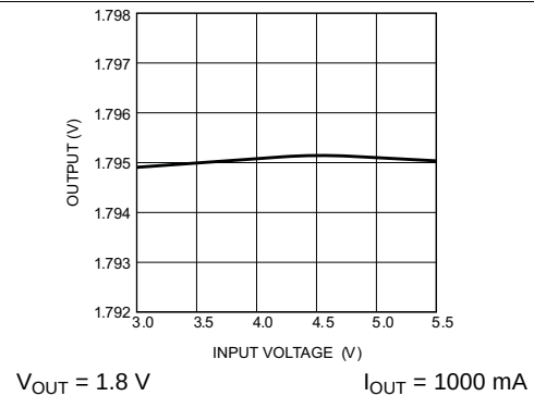
Figure 8. Line Regulation
