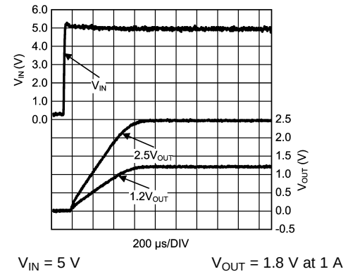
Figure 38. Start-Up (Soft Start)
