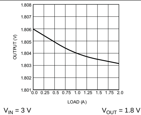
Figure 7. Load Regulation
