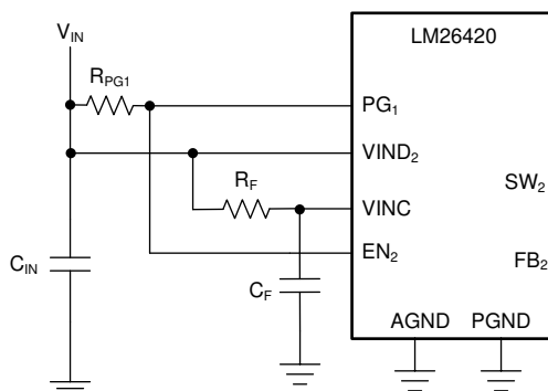
Figure 31. PG 1 Controlling V OUT2
