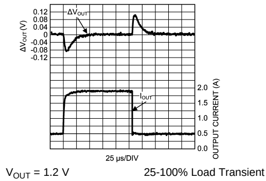
Figure 37. Load Transient Response
