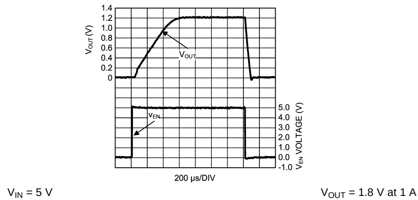
Figure 38. Start-Up (Soft Start)
