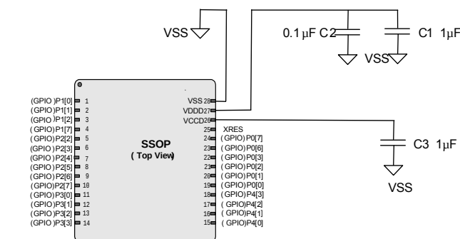
Figure 11. 28-SSOP Example
