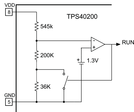
Figure 29. Undervoltage Lockout
