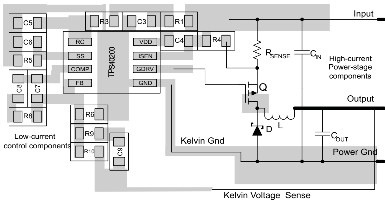
Figure 49. PC Board Layout Recommendations
