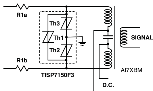
Figure 37. ISDN Protection
