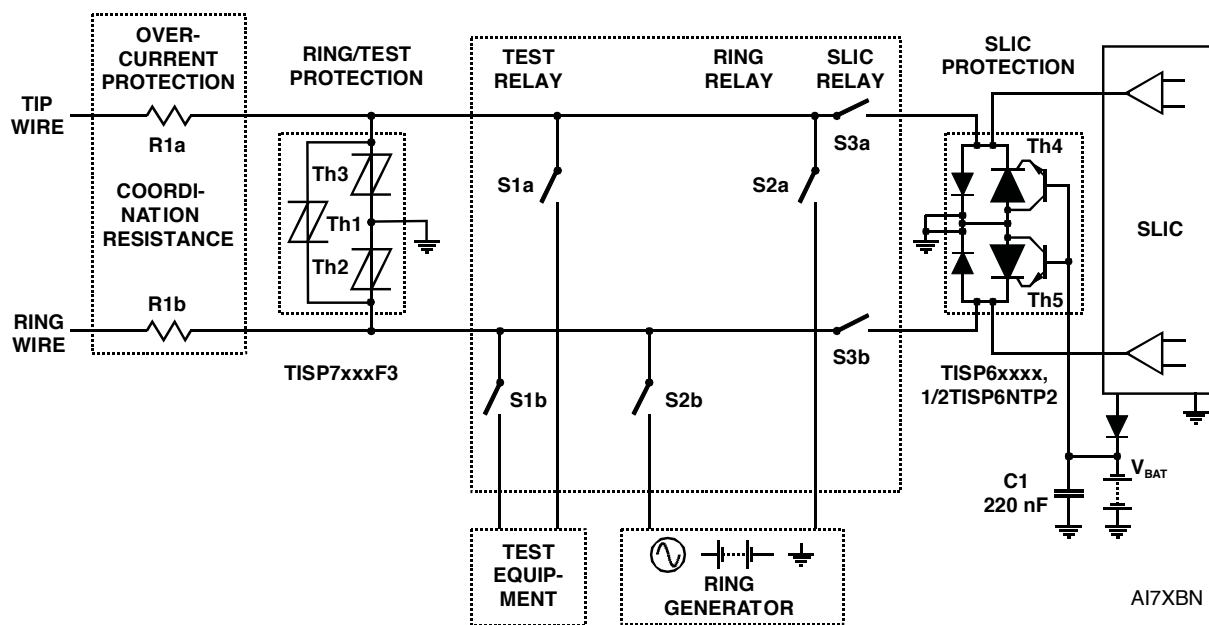
Figure 38. Line Card Ring/Test Protection
