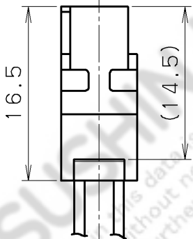
AFTER CABLE ASSEMBLY
