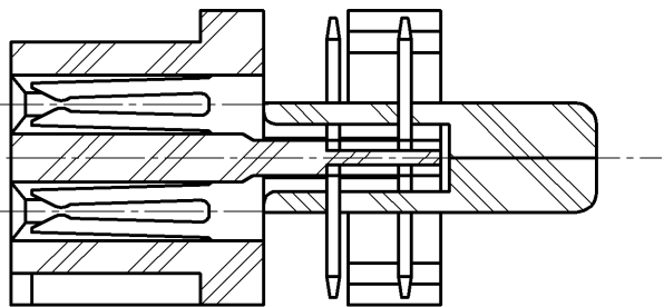
X-X SECTION (S=5/1)
