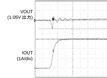
Fig.20 Transient Response 0→3A(0.6A/μs) ΔV=44mV
