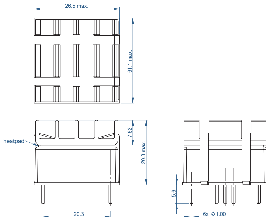
Dimension Drawing (mm) Heat sink version "/-HC"
