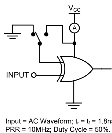
Figure 3. I_{CCD} Test Circuit
