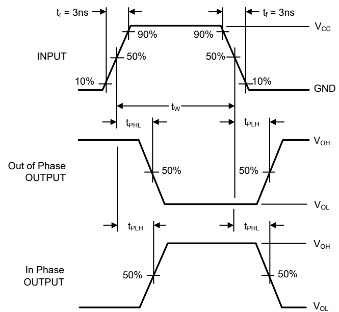
Figure 2. AC Waveforms
