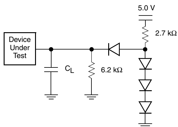
Figure 8. Test Setup
