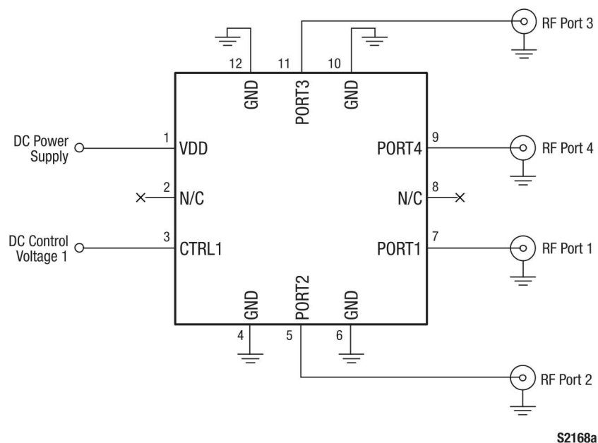
Figure 3. SKYA21026 Evaluation Board Schematic
