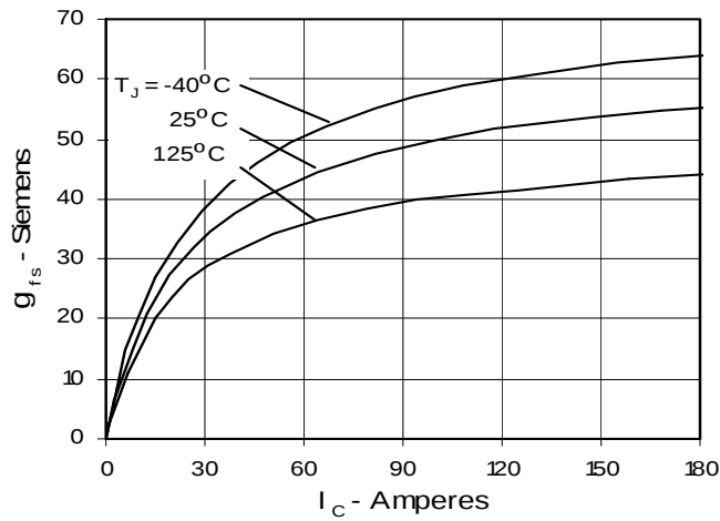
Fig. 7. Transconductance
