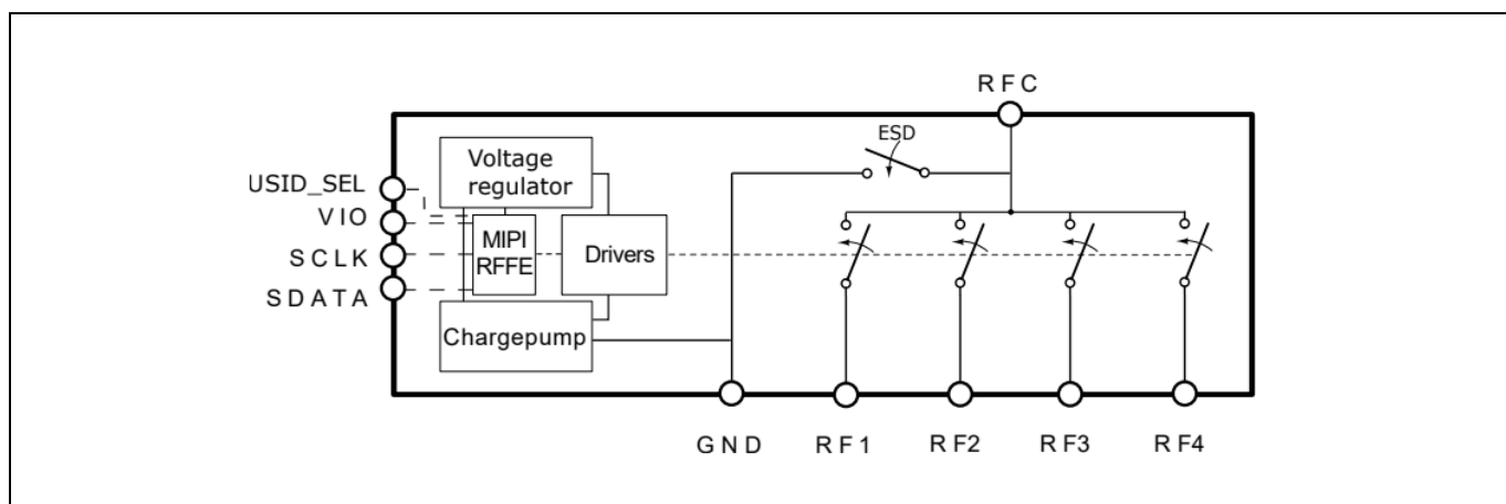
Figure 1 BGSA149M2N10 Block diagram
