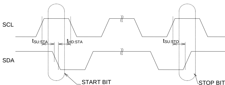
Figure 6. Start and stop condition
