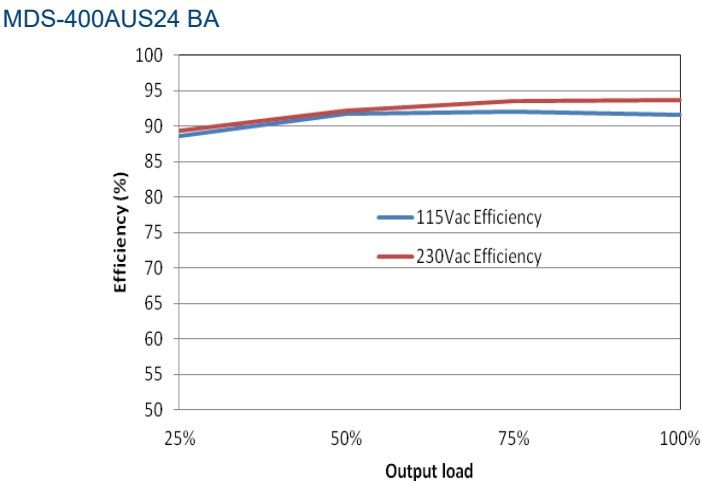
Fig.1-2 MDS-400AUS24 BA Efficiency versus output load
