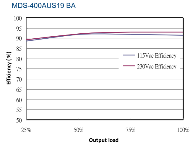
Fig.1-1 MDS-400AUS19 BA Efficiency versus output load
