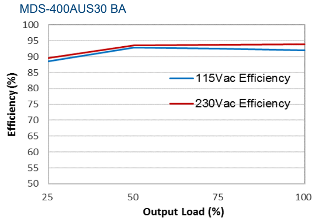
Fig.1-3 MDS-400AUS30 BA Efficiency versus output load
