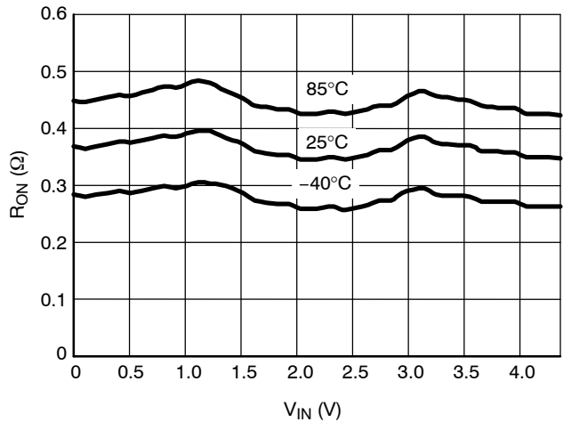
Figure 12. R_{ON} vs. V_{IN} vs. Temperature @ V_{CC} = 4.3 V
