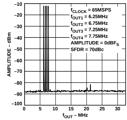
Figure 16. Four-Tone SFDR
