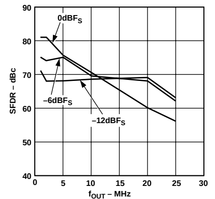
Figure 5. SFDR vs. f_{OUT} @ 65 MSPS
