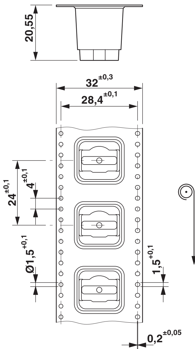
Dimensional drawing
