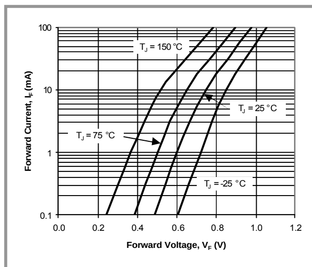
ig. 3. Forward Current vs. Forward Voltage
