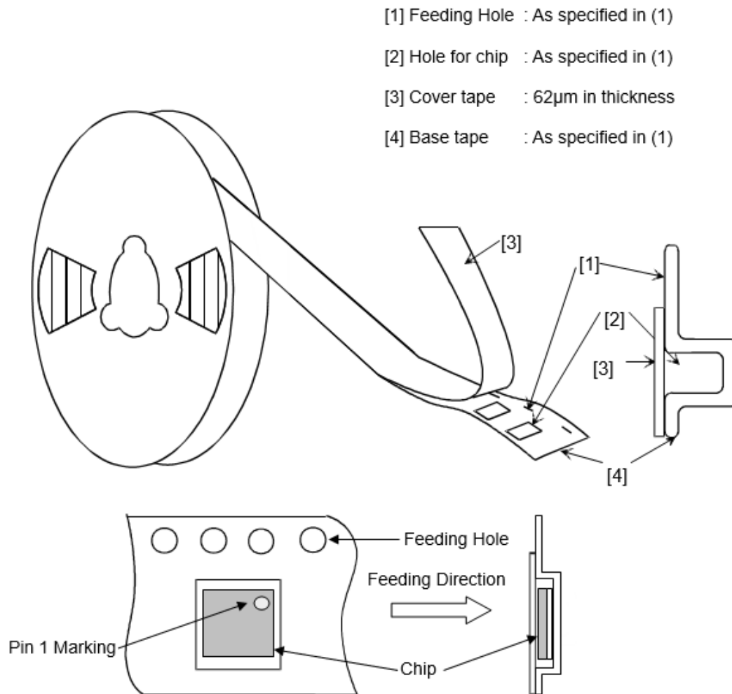
Figure 7.3 Taping Diagram
