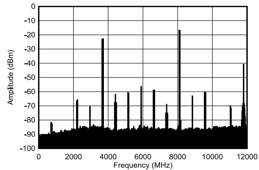
Figure 5-209. TX Dual Tone Output Spectrum at 8.11 GHz
