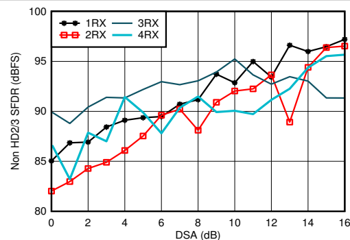
Figure 5-305. RX Non-HD2/3 vs DSA Setting at 0.8 GHz
