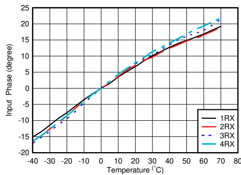
Figure 5-311. RX Input Phase vs Temperature and DSA at f_{\text{IN}} = 1.75 \text{ GHz}
