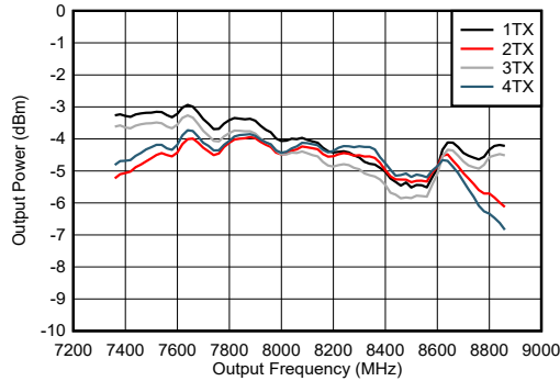
Figure 5-184. TX Output Power vs Frequency at 8.11 GHz
