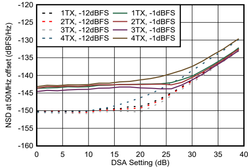
Figure 5-220. TX NSD vs DSA Setting at 8.11 GHz
