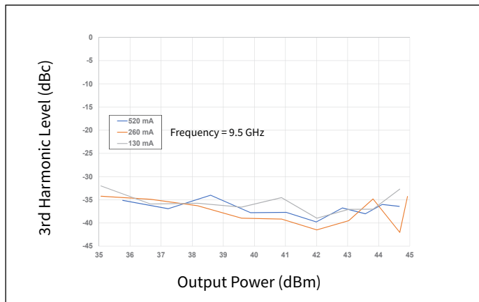
Figure 33. 3rd Harmonic vs Output Power as a Function of I_{DQ}
