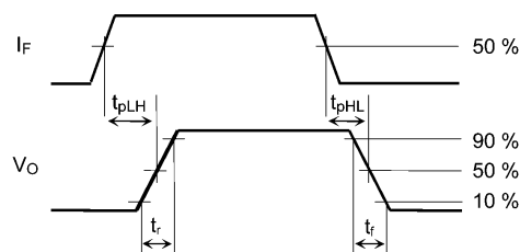
Fig. 12.1.5 Switching Time Test Circuit and Waveform
