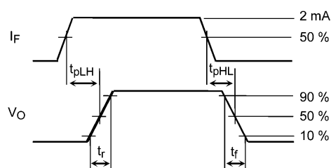
Fig. 12.1.6 Switching Time Test Circuit and Waveform
