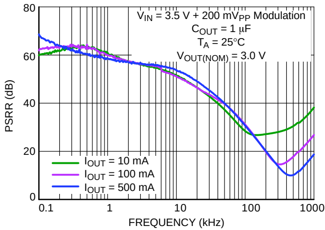
Figure 27. PSRR vs. Frequency &amp; Output Current
