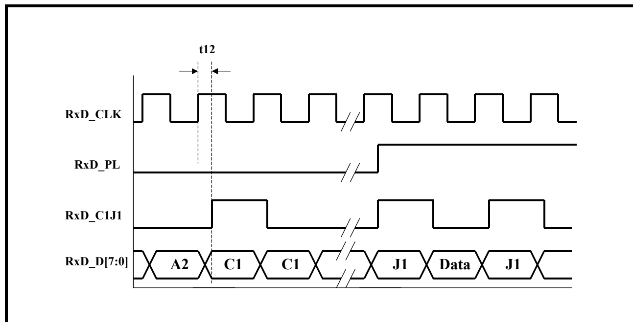
FIGURE 18. AN ILLUSTRATION OF THE WAVEFORMS OF THE SIGNALS THAT ARE OUTPUT VIA THE RECEIVE STS-1/STM-0 TELECOM BUS INTERFACE
