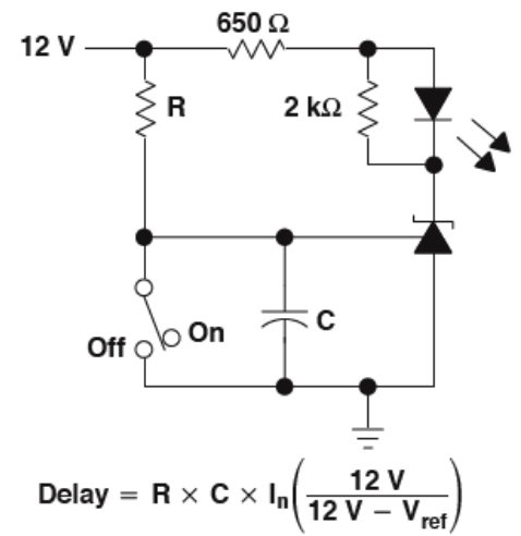
Figure 14: Delay Timer
