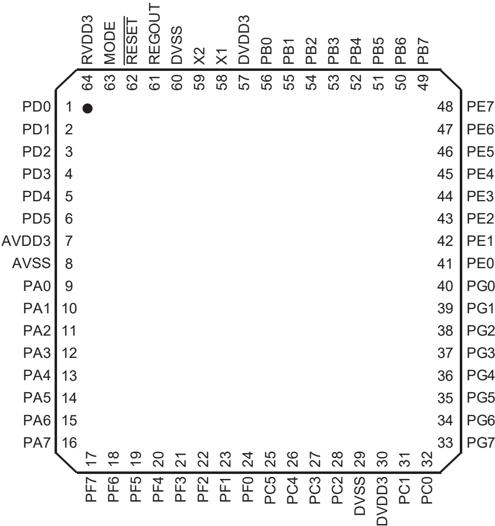
Figure 1-2 Pin Layout (LQFP64 TOP VIEW)
