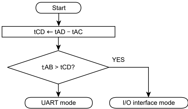
Figure 17-8 Serial operation mode determination flowchart
