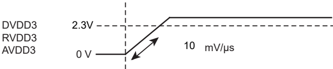
Figure 20-2 Voltage level of power supply at power-on
