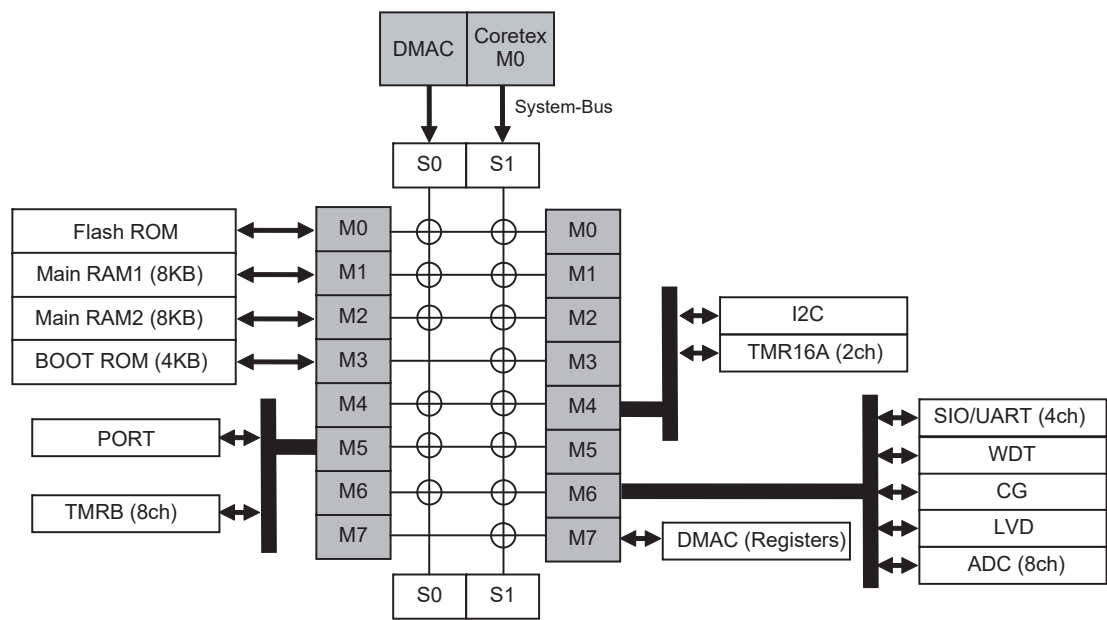
Figure 4-3 TMPM037FWUG (Single boot mode)
