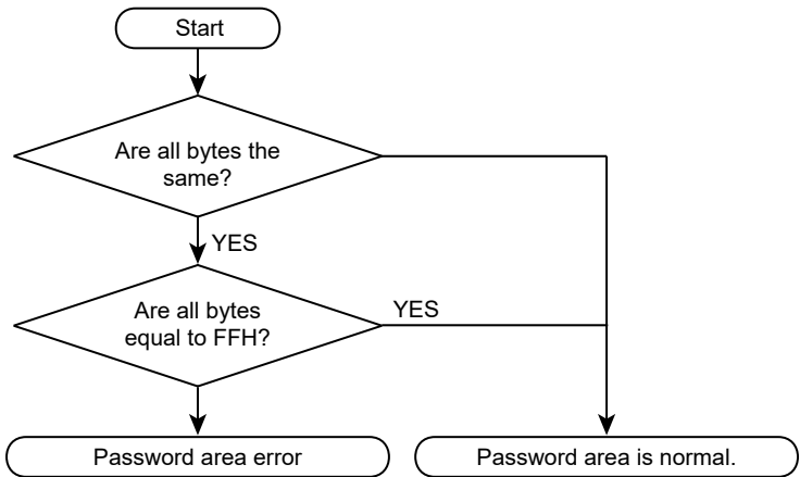
Figure 17-9 Password area check flowchart
