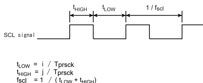
Figure 13-4 Clock source
