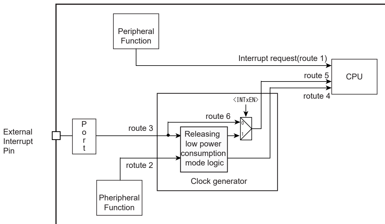
Figure 7-1 Interrupt Route
