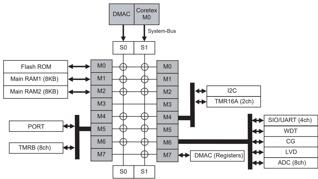
Figure 4-2 TMPM037FWUG (Single chip mode)
