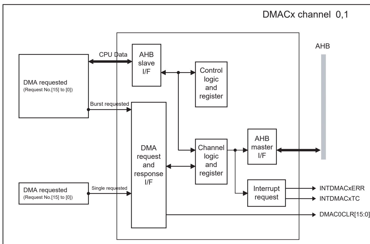
Figure 8-1 DMAC Block diagram
