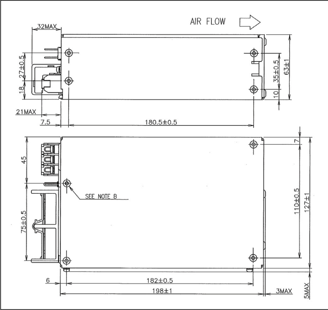
Outline Drawing RWS1000B
