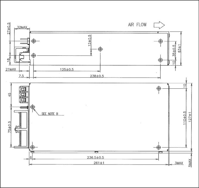
Outline Drawing RWS1500B
