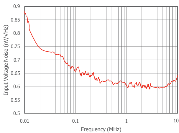
Input Voltage Noise at V_S = 5\text{V} ( >10\text{kHz} )
