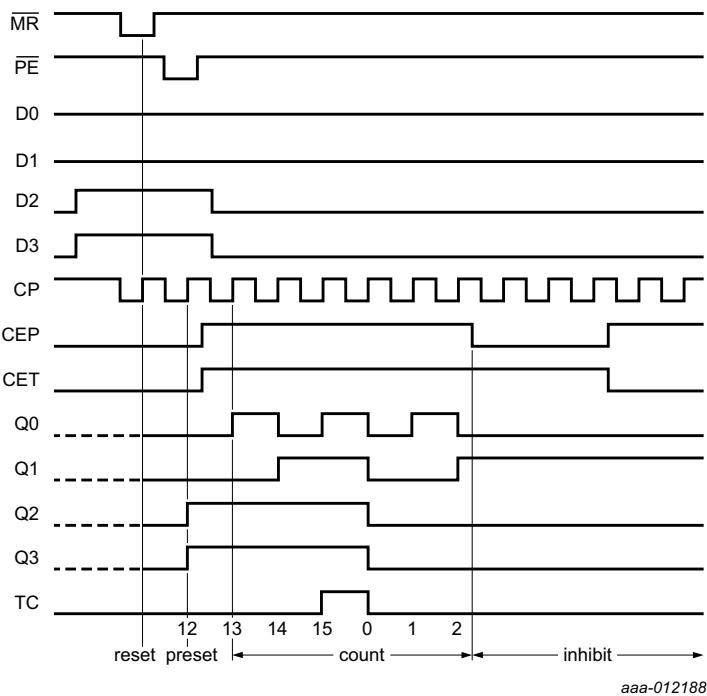
Sequence reset outputs to zero; preset to binary 12; count to 13, 14, 15, zero, one and two; inhibit.
