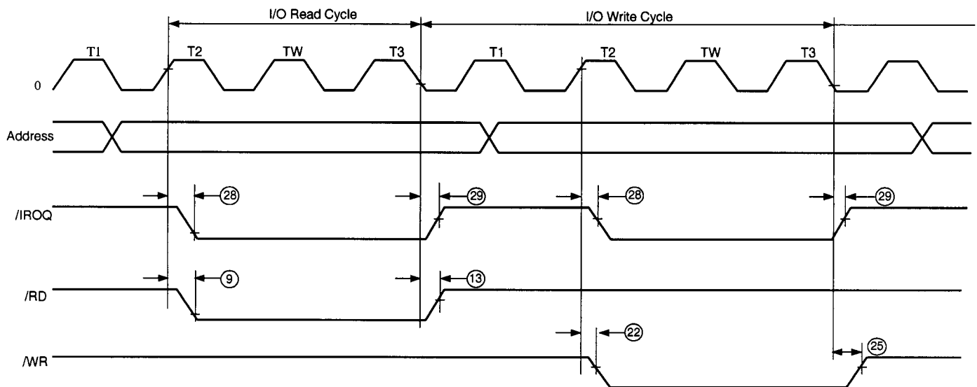
Figure 6. CPU Timing
