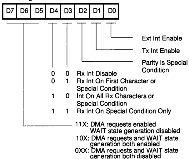
Write Register 1
