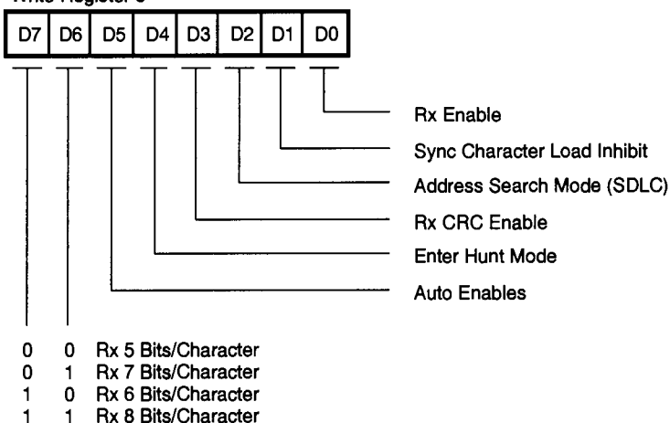
Write Register 3
