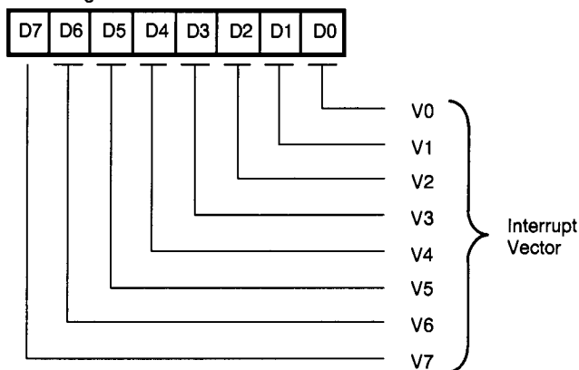
Write Register 2
