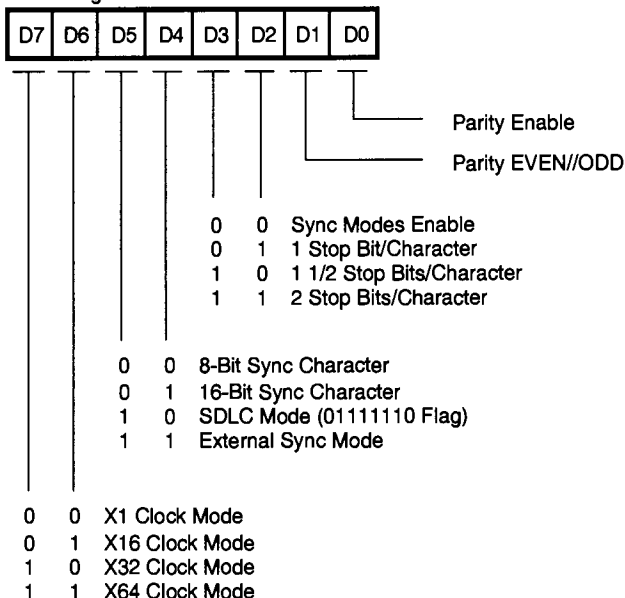
Write Register 4
