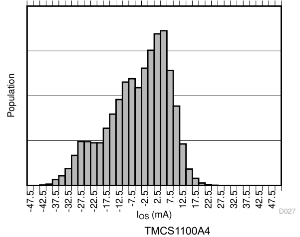
Figure 7-8. Input Offset Current Production Distribution
