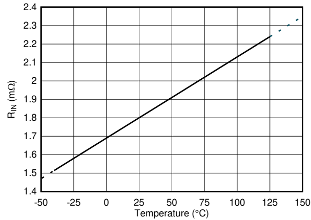
Figure 7-21. Input Conductor Resistance vs. Temperature
