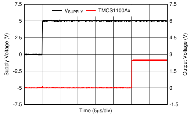
Figure 7-20. Startup Transient Response
