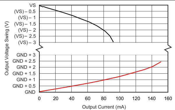
Figure 7-12. Output Swing vs. Output Current
