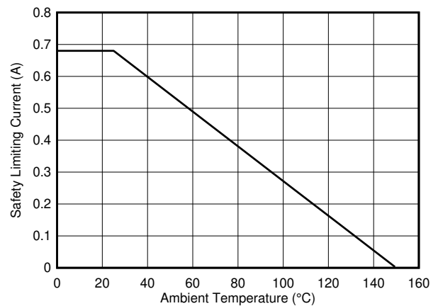
Figure 7-23. Thermal Derating Curve for Safety-Limiting Current, Side 2
