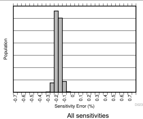
Figure 7-4. Sensitivity Error Production Distribution
