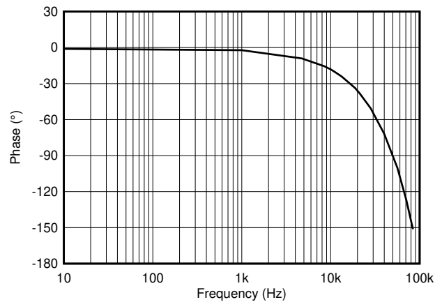
Figure 7-10. Phase vs. Frequency, All Gains
