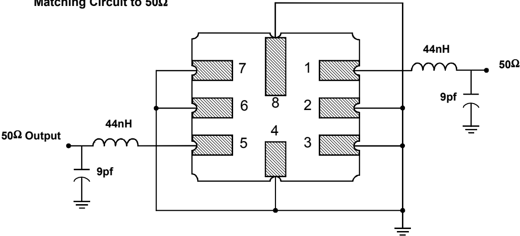
Matching Circuit to 50Ω
