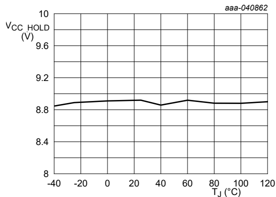
Fig. 4. V CC_HOLD vs. junction temperature
