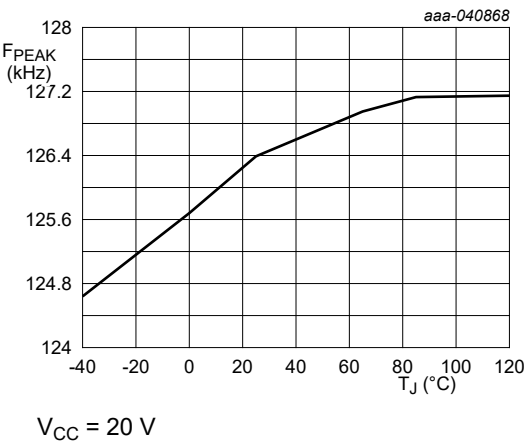
Fig. 10. F_{PEAK} vs. junction temperature
