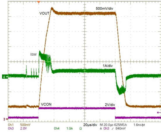
Figure 40. Transient Response V_{OUT} vs V_{CON} R_L = 10\text{ }\Omega , V_{OUT} = 0.4\text{ V to } 3.5\text{ V} , PV_{IN} = 3.9\text{ V}
