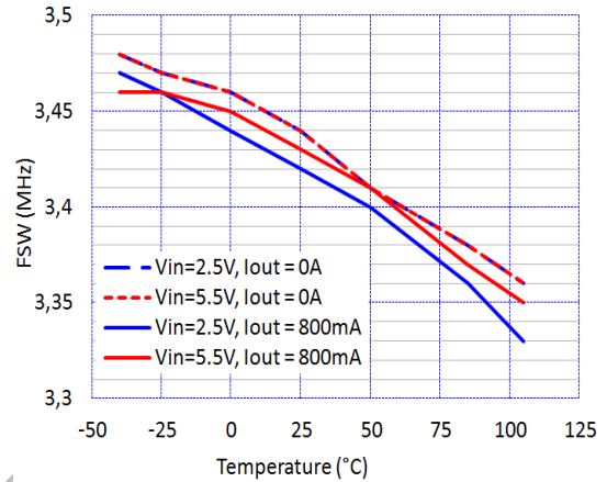
Figure 12. 3.429 MHz Switching Frequency Variation ( F_{sw} ) vs. Temperature ( L = 1\text{ }\mu\text{H} )
