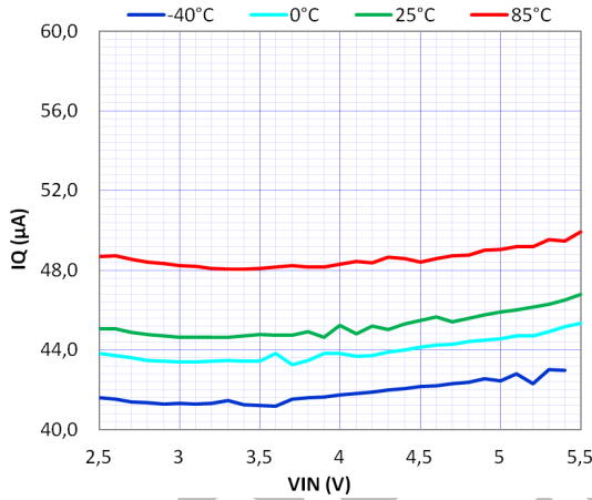
Figure 7. Quiescent Current vs. Input Voltage ( EN = \text{High} , V_{CON} = 0.8\text{ V} , V_{OUT} = 2\text{ V} )
