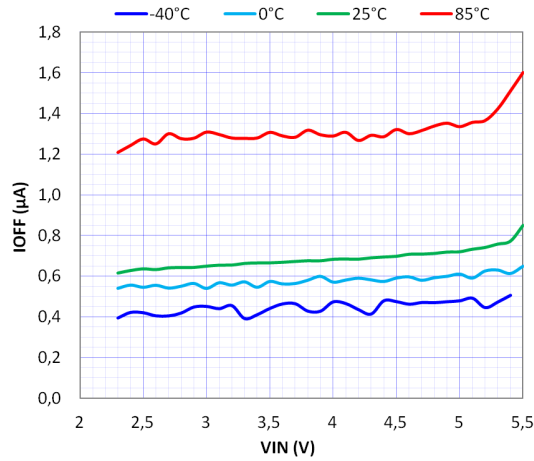
Figure 5. Shutdown Current vs Input Voltage ( EN = \text{Low} , V_{CON} = 0\text{ V} )
