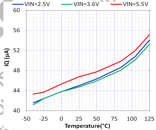
Figure 8. Quiescent Current vs Temperature ( T_A ) ( EN = \text{High} , V_{CON} = 0.8\text{ V} , V_{OUT} = 2\text{ V} )
