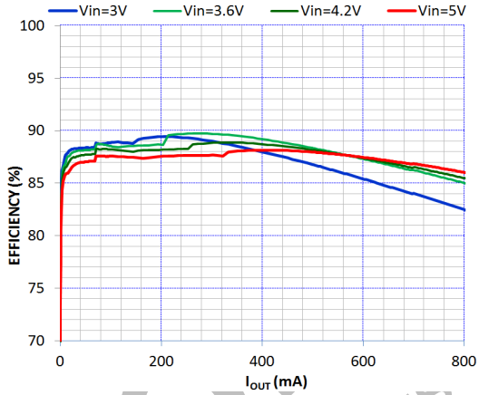
Figure 18. Efficiency vs Output Current vs PV_{IN} @25°C, F_{sw} = 6\text{ MHz} , V_{OUT} = 1.8\text{ V}
