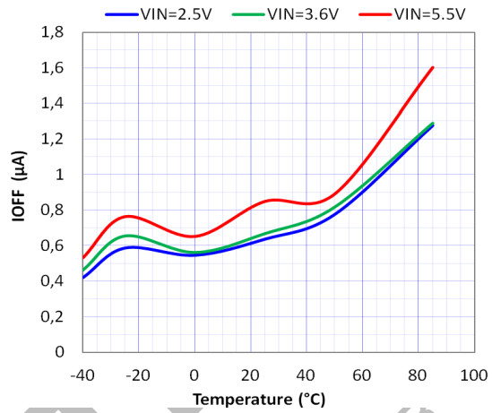
Figure 6. Shutdown Current vs Temperature ( T_A ) ( EN = \text{Low} , V_{CON} = 0\text{ V} )
