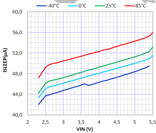
Figure 9. Sleep Mode Current vs. Input Voltage ( EN = \text{High} , V_{CON} = 0\text{ V} , V_{OUT} = 0\text{ V} )
