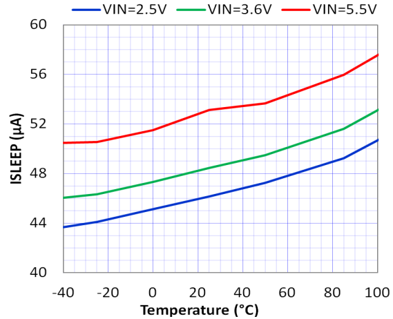
Figure 10. Sleep Mode Current vs. Temperature ( T_A ) ( EN = \text{High} , V_{CON} = 0\text{ V} , V_{OUT} = 0\text{ V} )
