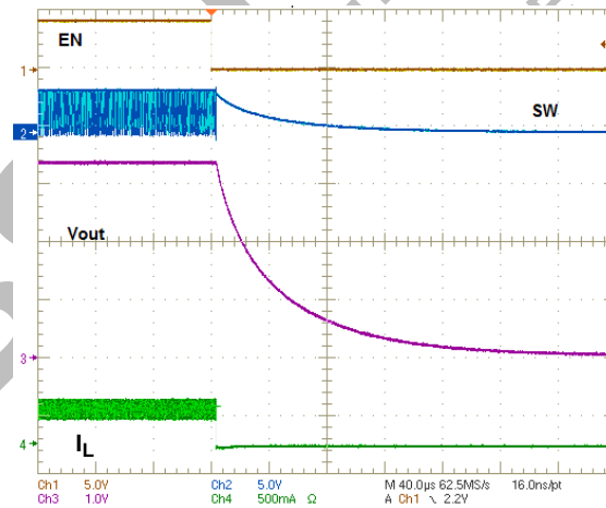
Figure 48. Power-down Transient Response PV_{IN} = 3.7\text{ V} , V_{out} = 3.4\text{ V} , R_L = 10\text{ }\Omega
