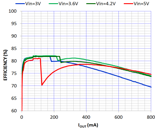
Figure 16. Efficiency vs Output Current vs PV_{IN} @25°C, F_{sw} = 6\text{ MHz} , V_{OUT} = 0.8\text{ V}
