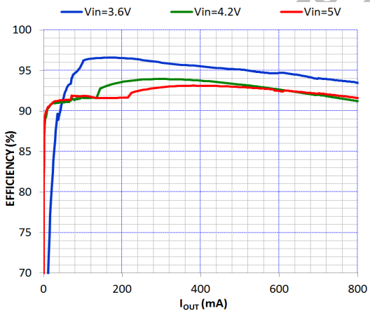
Figure 20. Efficiency vs Output Current vs PV_{IN} @25°C, F_{sw} = 6\text{ MHz} , V_{OUT} = 3.3\text{ V}
