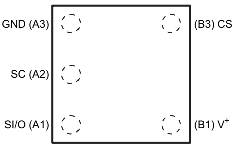
Figure 3. 5-Bump DSBGA – Top View See Package Number YTA0005
