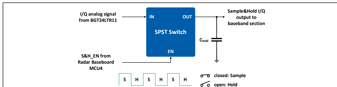
Figure 9 S&H circuitry
